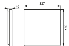
VARSO LED 24W...L
