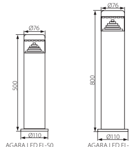
AGARA LED EL-50
