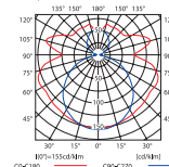
ALDO 236 curve of intensity distribution / Lichtverteilungskurve η = 94%
