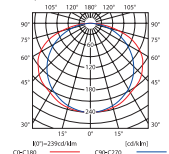
ALDO 236R curve of intensity distribution / Lichtverteilungskurve η = 82%
