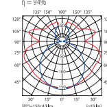
ALDO 258 curve of intensity distribution / Lichtverteilungskurve η = 94%
