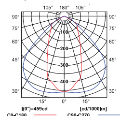
AVIA MTH-478/400W-B
